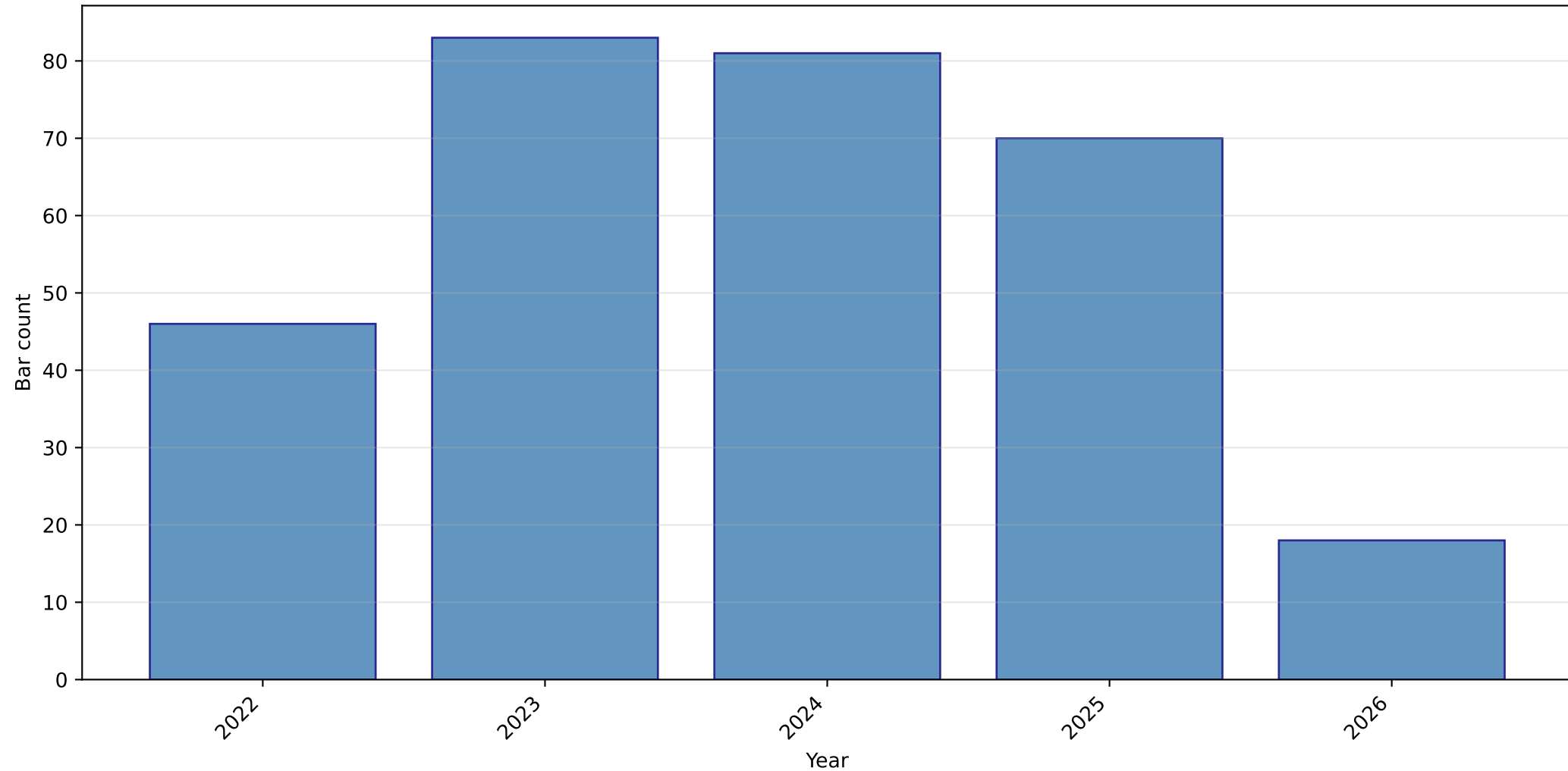
Regime 40 — bar counts by year (UTC) EURUSD · 60-minute bars (H1) · n=25,000 bars
